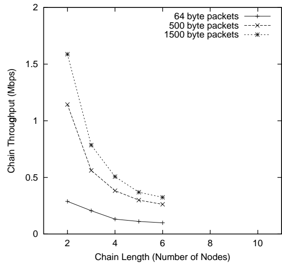
Figure 6: Real hardware throughput achieved along a chain of nodes, as a function of the chain length. Each node was placed at the maximum distance from the previous that allowed low-loss communications. Hardware parameters were set to mimic the simulation parameters as much as possible.
