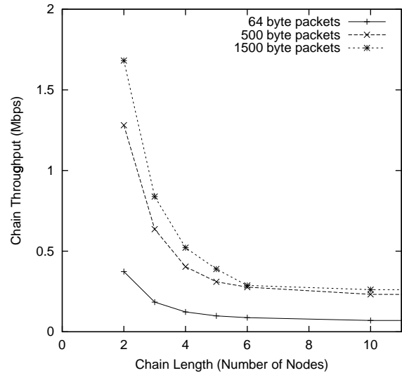
Figure 3: Throughput achieved along a chain of nodes, as a function of the chain length. The nodes are 200 meters apart. The first node originates packets as fast as 802.11 allows, to be forwarded along the chain to the last node. The throughputs for chains of 20 and 50 nodes are the same as for 10 nodes.
